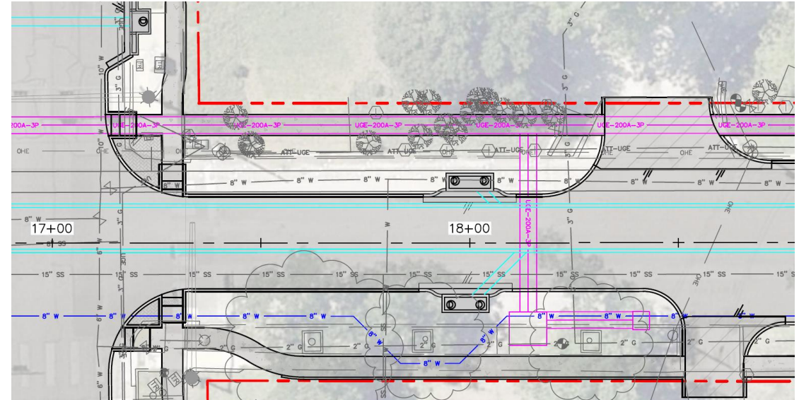
Proposed Shared Duct Bank
