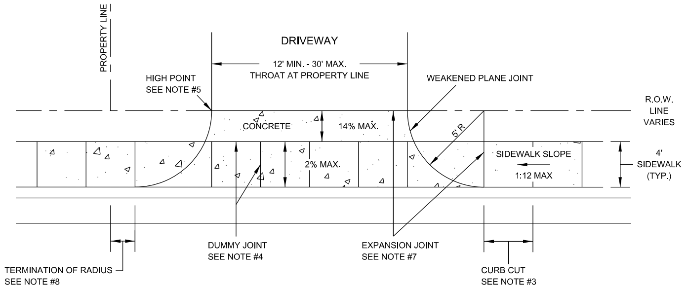
RADIUS PLAN VIEW
